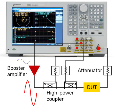
Figure 5. Configuration example using direct receiver access
