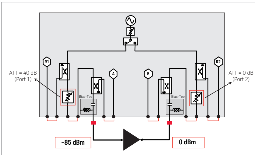
Figure 9. Uncoupled output power with independent source attenuators
