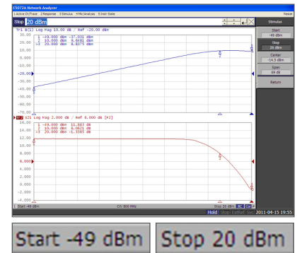
Figure 3. Widest power sweep range n class (ex. settable from -49 dBm to +20 dBm)
